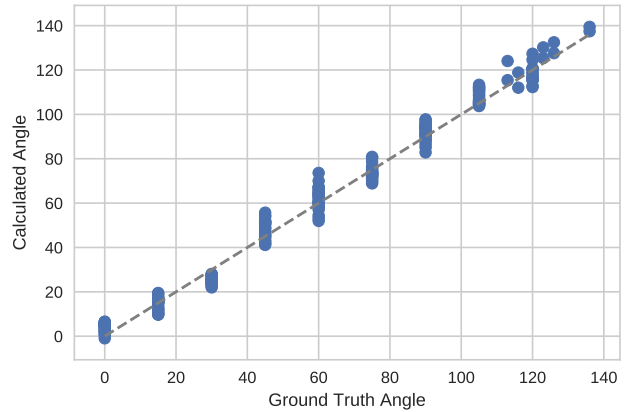
Figure 14: Comparison of Ground Truth Angle and Calculated Angle
