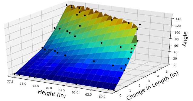
Figure 3: Change in length to angle model with height as a parameter.
