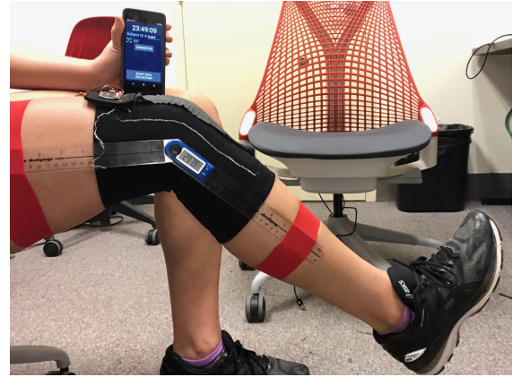
Figure 13: User Study Setup
