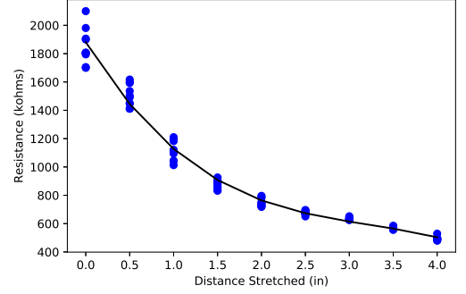
Figure 4: Fabric Resistance to Stretch Distance
