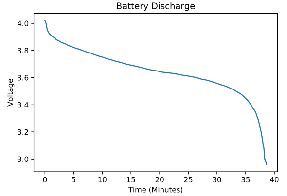
Figure 15: Voltage of Battery Over Time
