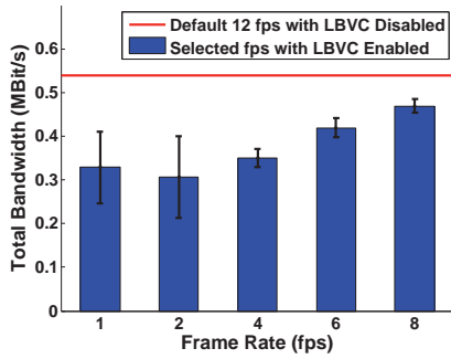
Figure 8: Bandwidth Usage vs. Frame Rate on Galaxy Nexus.
