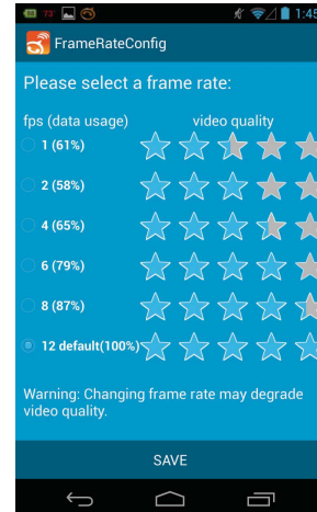
Figure 7: The Interface.
