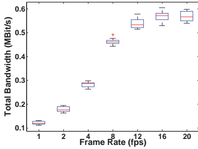
Figure 1: Total Bandwidth vs. Frame Rate on Galaxy Nexus.
