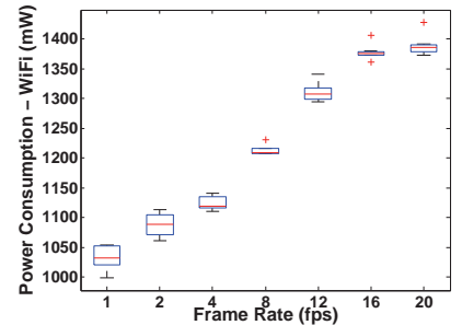
Figure 3: Power Consumption vs. Frame Rate on Galaxy Nexus in a WiFi Network.
