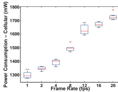
Figure 2: Power Consumption vs. Frame Rate on Galaxy Nexus in a Cellular Network.
