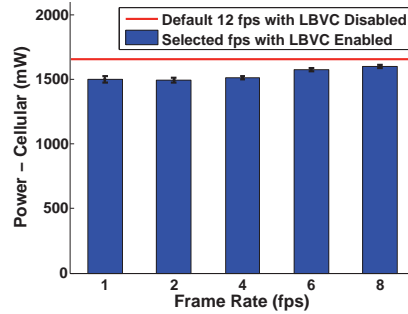
Figure 9: Power Consumption vs. Frame Rate in a Cellular Network on Galaxy Nexus.
