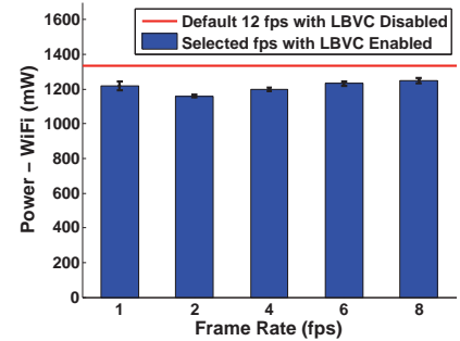
Figure 10: Power Consumption vs. Frame Rate in a WiFi Network on Galaxy Nexus.
