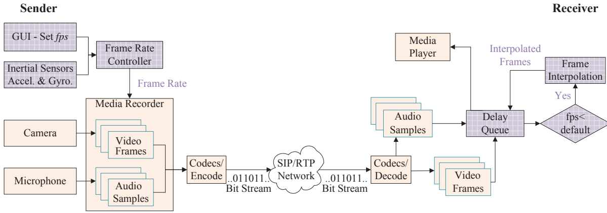
Figure 5: LBVC Architecture.
