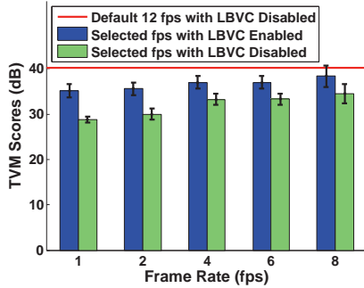
Figure 12: TVM Scores vs. Frame Rate. Error Bars indicate the Standard Deviations.
