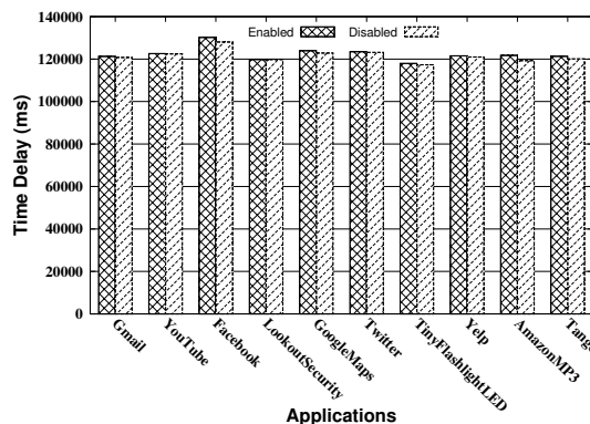
Figure 11. Application Delay.
