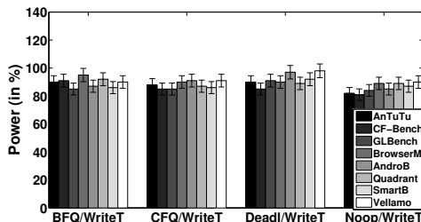
Figure 4. Power for Write-through Cache. The measurements are obtained while keeping default queue depth (128). The results are compared to the power levels with default configurations in Figure 2 that are baseline values.
