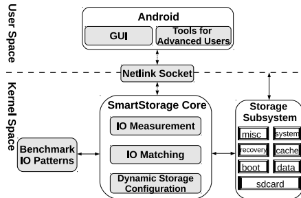
Figure 5. SmartStorage Architecture.
